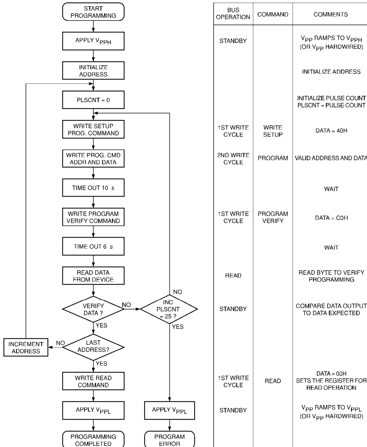
Figure 7. Programming Algorithm (1)
