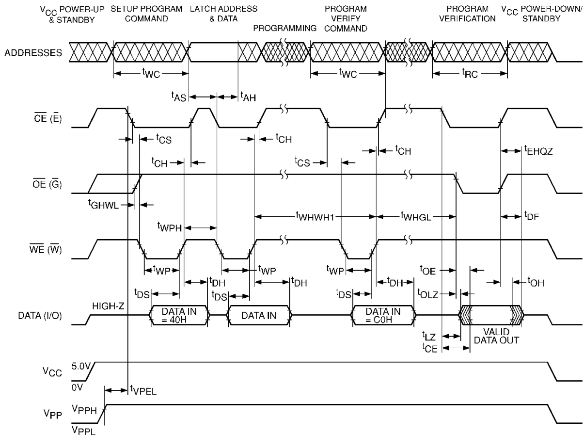
Figure 6. A.C. Timing for Programming Operation
