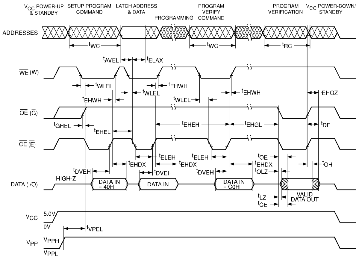
Figure 8. Alternate A.C. Timing for Programming Operation
