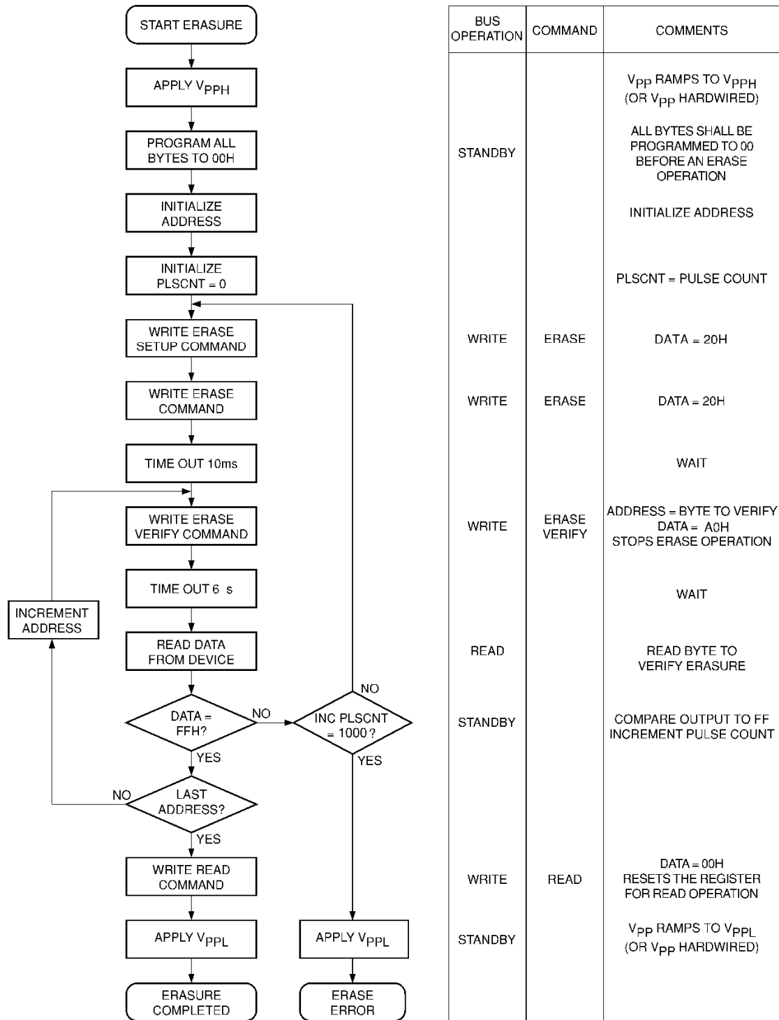
Figure 5. Chip Erase Algorithm (1)
