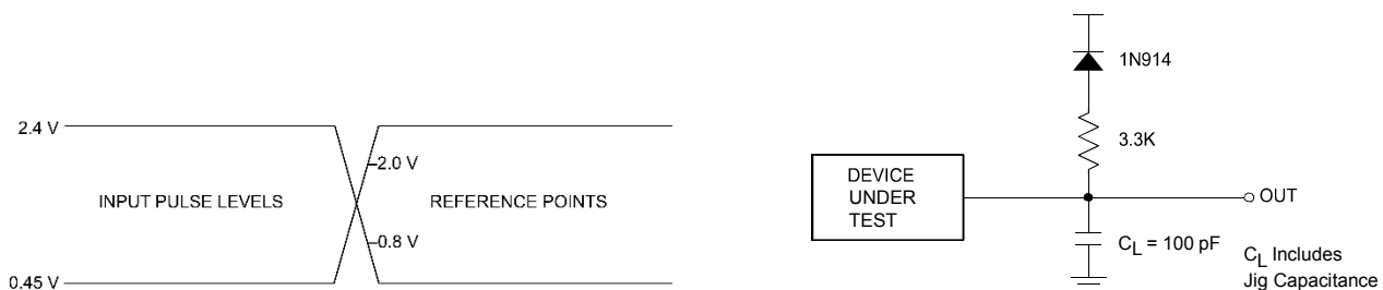
Figure 1. A.C. Testing Input/Output Waveform (3)(4)(5)
