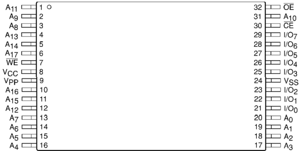
TSOP
