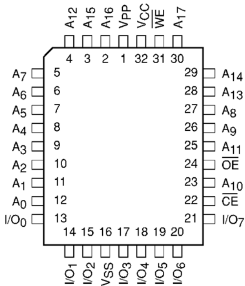
PLCC Package
