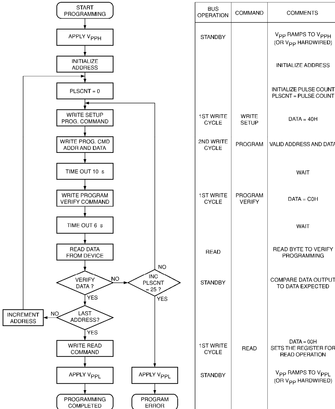
Figure 7. Programming Algorithm (1)
