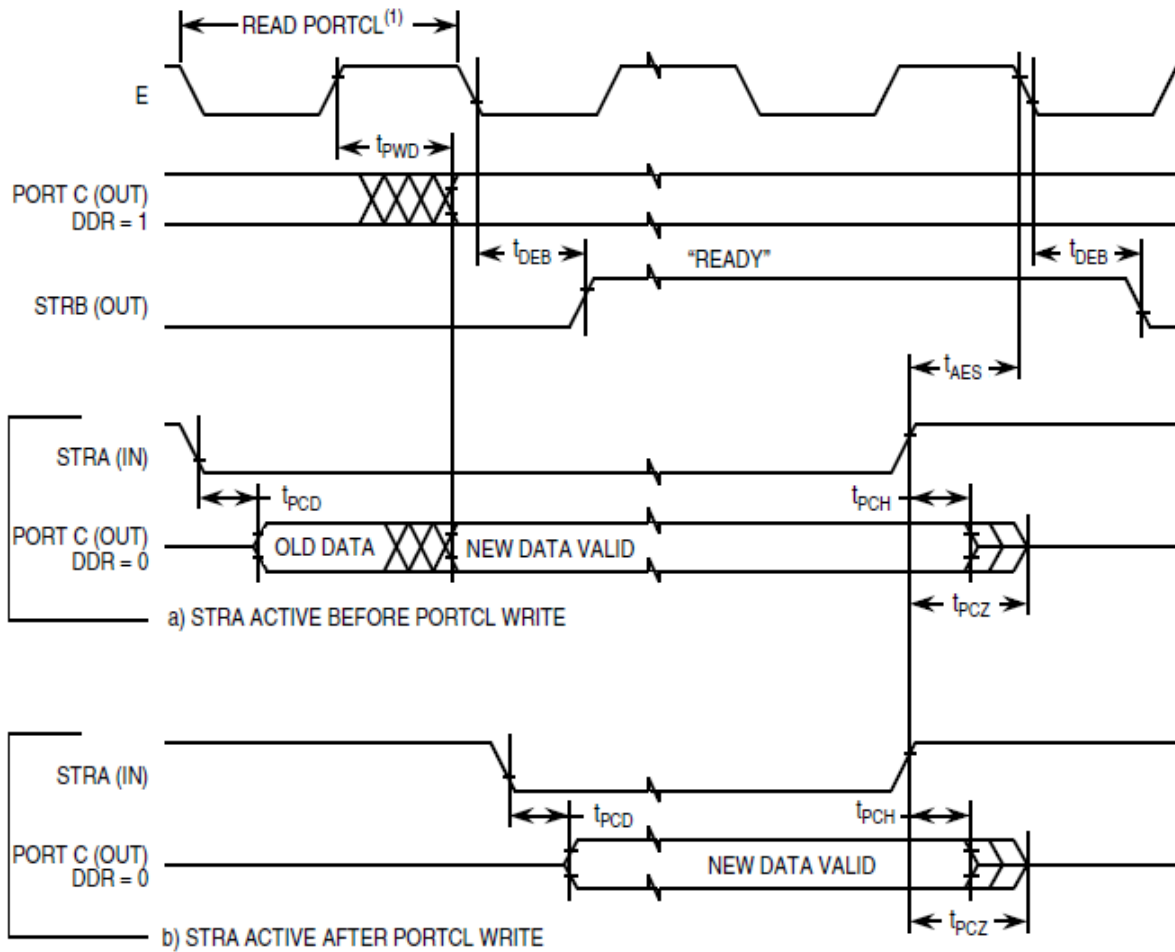
State Variation of Output Handshake Timing Diagram (STRA Enables Output Buffer)
