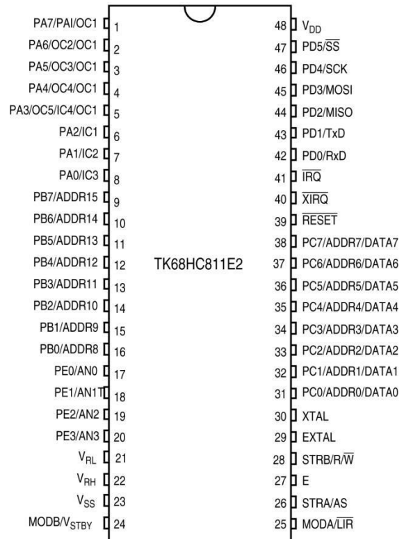
Pin Assignments for 48-Pin DIP
