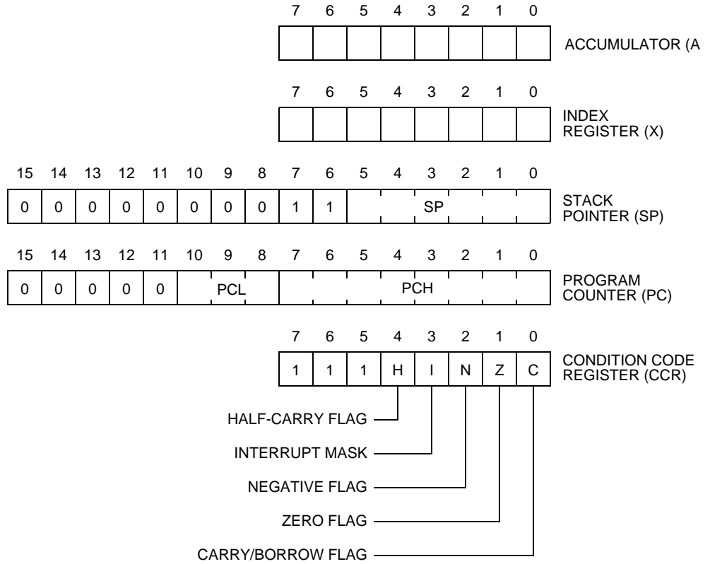
Figure 3-1. Programming Model
