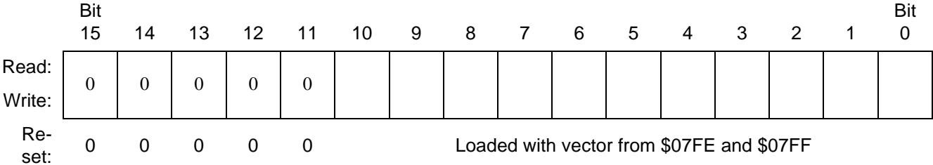
Figure 3-5. Program Counter (PC)
