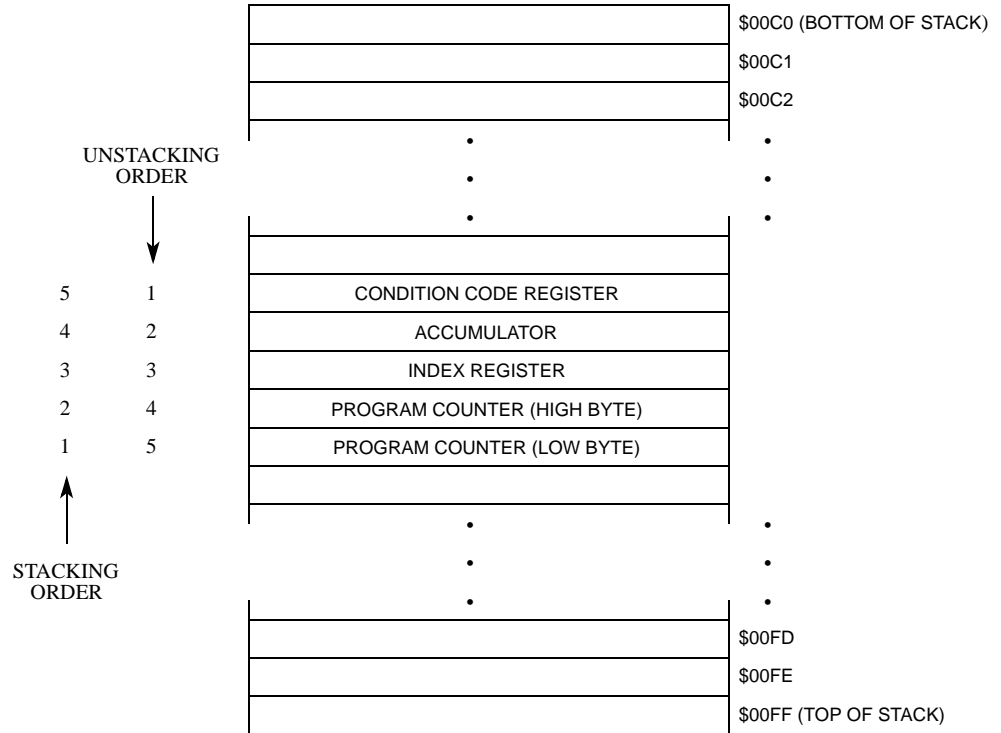
Figure 4-3. Stacking Order
