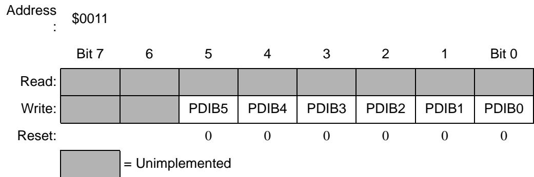
Figure 7-6. Pulldown Register B (PDRB)
