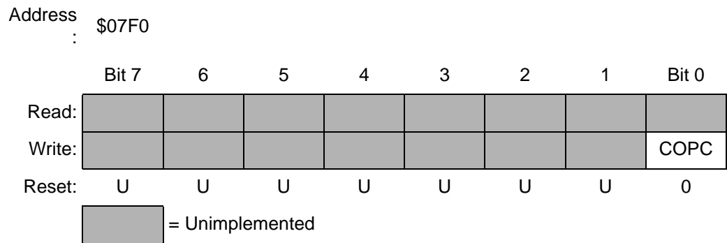
Figure 8-4. COP Register (COPR)
