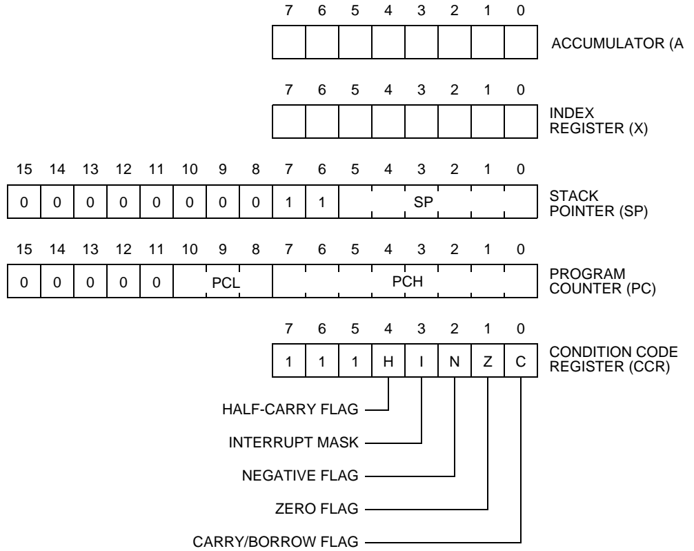
Figure 3-1. Programming Model
