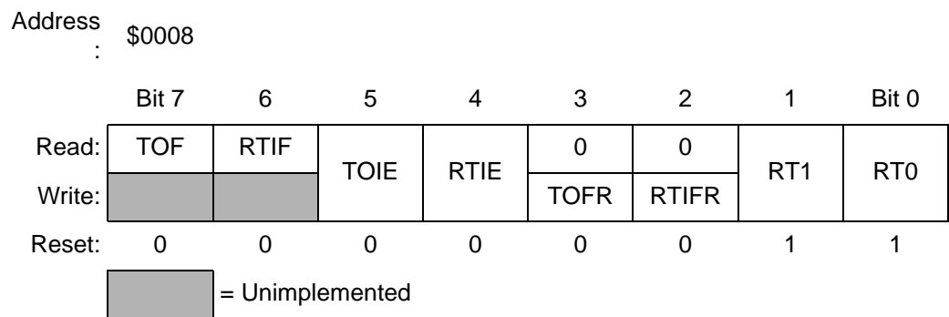
Figure 8-2. Timer Status and Control Register (TSCR)
