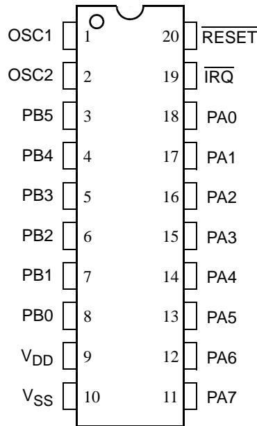
Figure 1-2. Pin Assignments
