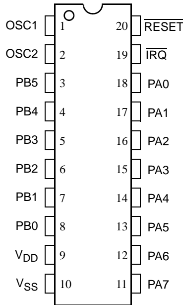
Figure 1-2. Pin Assignments
