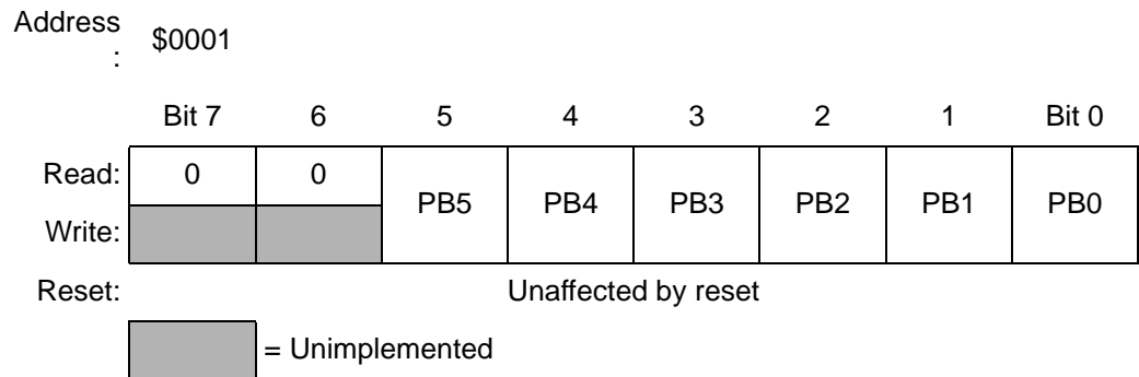
Figure 7-4. Port B Data Register (PORTB)
