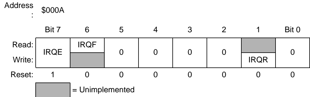
Figure 4-2. IRQ Status and Control Register (ISCR)
