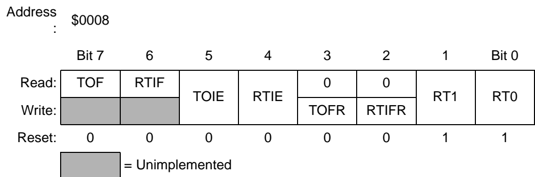
Figure 8-2. Timer Status and Control Register (TSCR)
