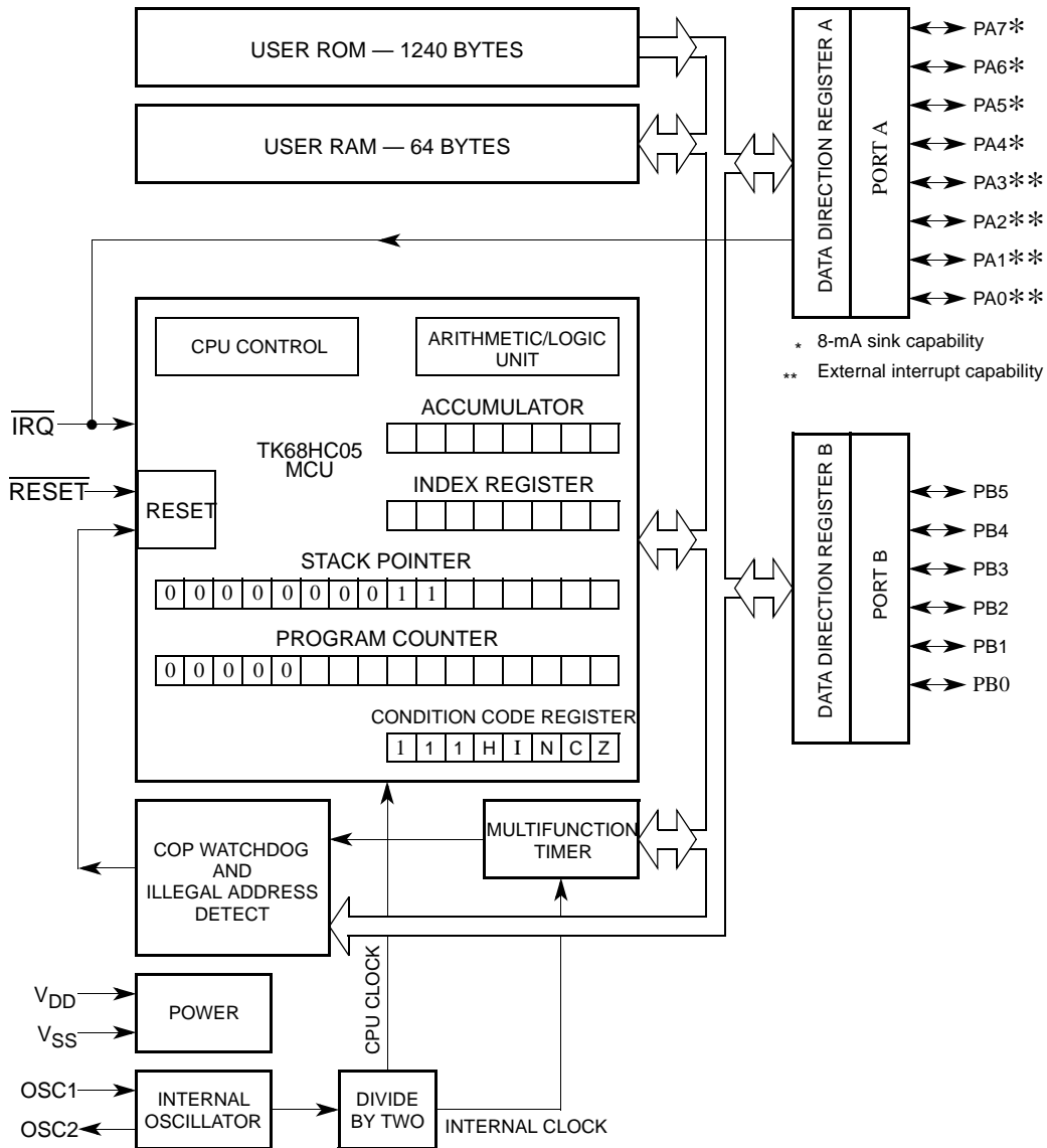
Figure 1-1. TK68HC05J1A Block Diagram
