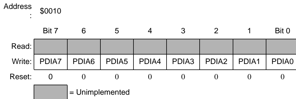
Figure 7-2. Pulldown Register A (PDRA)
