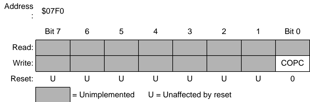
Figure 5-1. COP Register (COPR)
