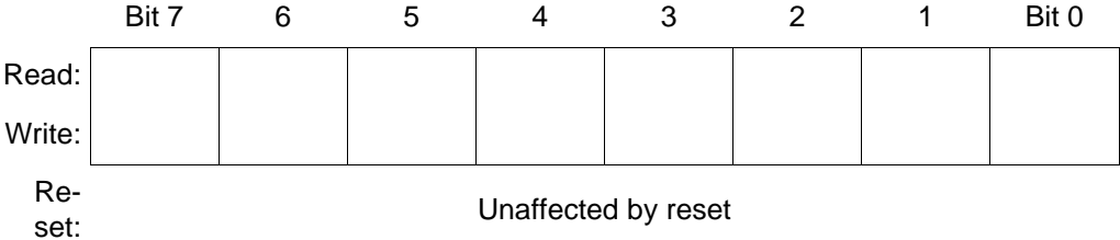
Figure 3-2. Accumulator (A)
