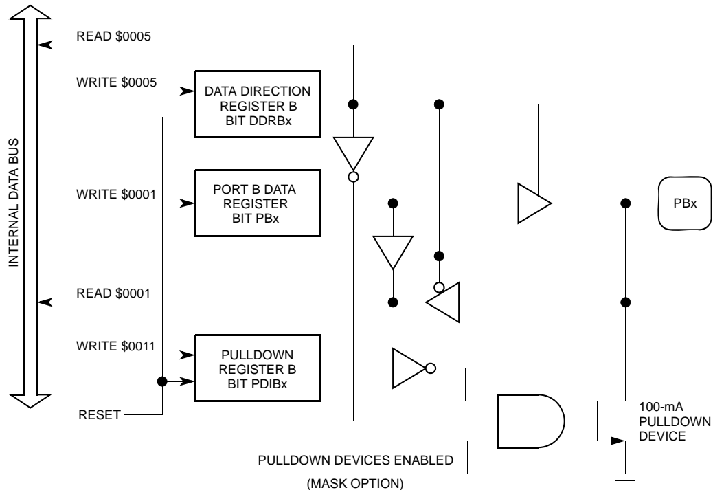
Figure 7-7. Port B I/O Circuit
