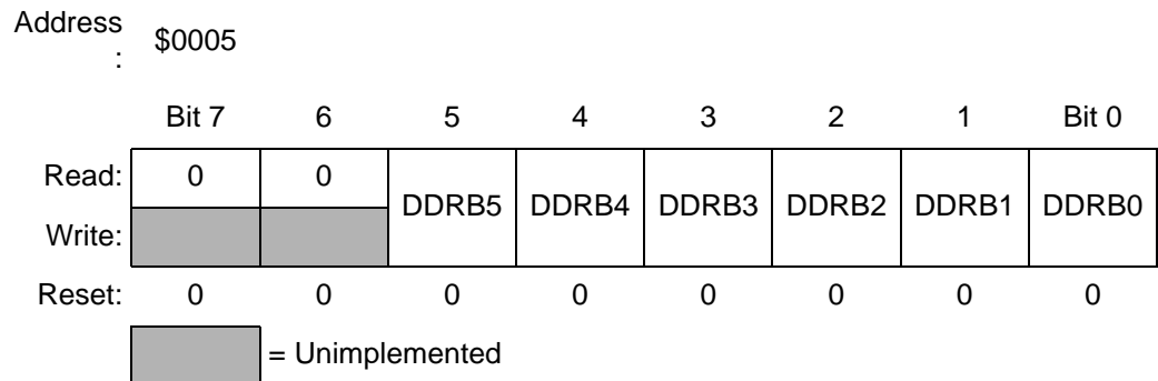
Figure 7-5. Data Direction Register B (DDRB)
