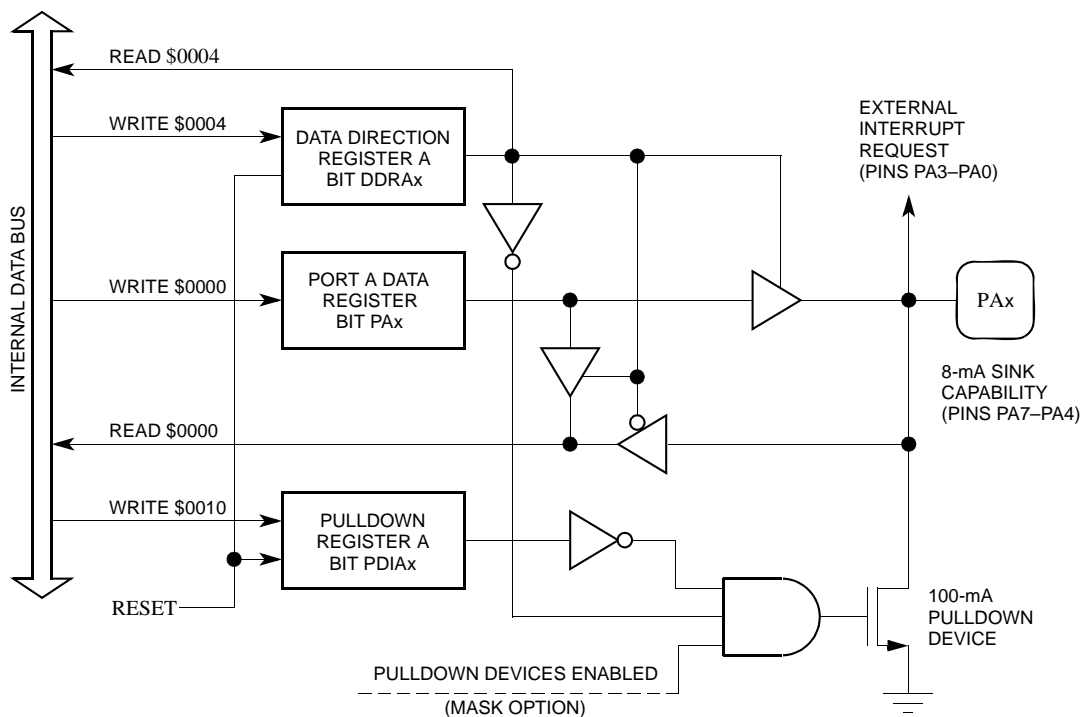
Figure 7-3. Port A I/O Circuit
