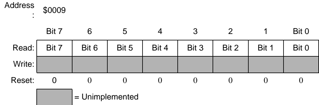
Figure 8-3. Timer Counter Register (TCNTR)
