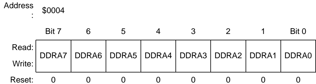
Figure 7-1. Data Direction Register A (DDRA)
